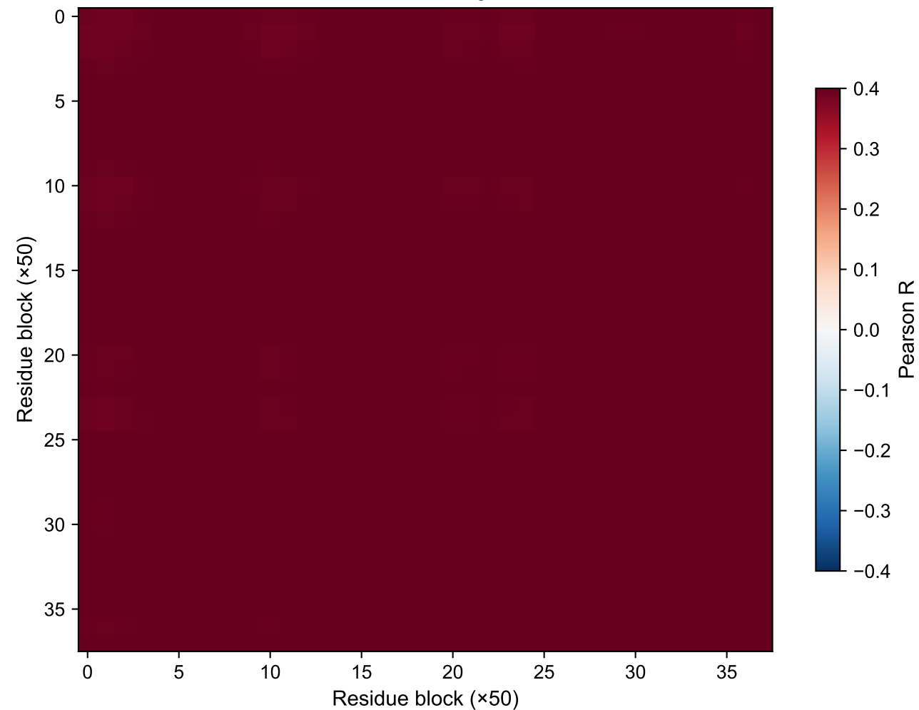
HYDROMORPHONE: Highest RMSD
